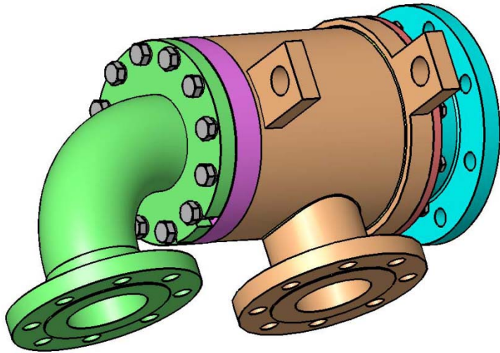
Three-dimensional Drawing of TSXF150-100 Rotary Joint
